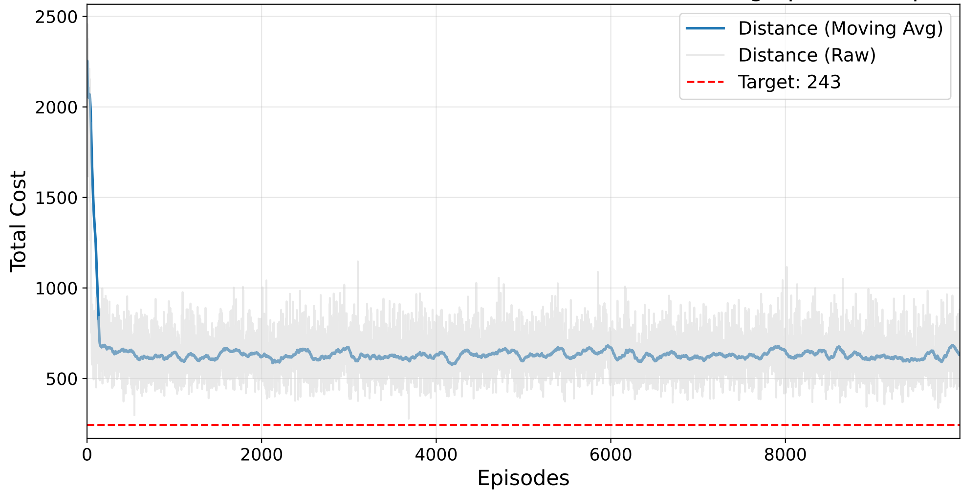
Final GAUSSIAN PROCESS Masked AutoRL-SOP Training - prob.42.sop
